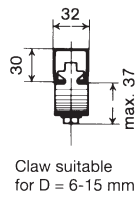
View without I-beam
